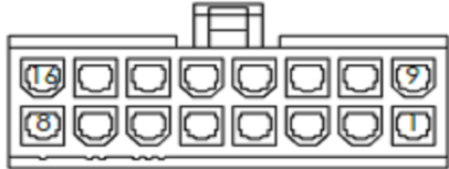
39-01-2160 CONNECTOR VIEWED FROM CONNECTION SIDE
