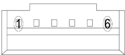
PHR-6 CONNECTOR VIEWED FROM CONNECTION SIDE
